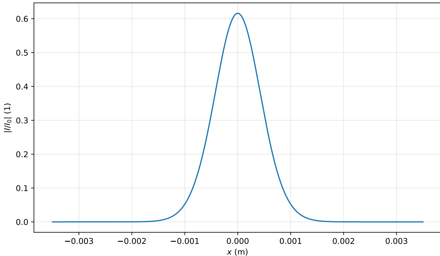
Intensity profile I(x, y = 0, z = 1.911m)/I_0 , P_{in}=0.2P_{cr} , artificial time
